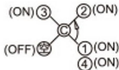
SCHEMATIC (NON-SHORTING)
